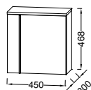
Base unit for handwash basin, RH 45 x 30 cm 1 soft-close door and 1 shelf EB3045D Starting at €370 incl. VAT and €0.50 eco-contribution
