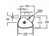
Handwash basin 45 x 36 cm EGK112 €250 incl. VAT
