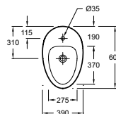
Smooth-sided floor bidet 60 x 39 cm EBD0002 €330 incl. VAT
