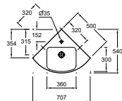
Corner washbasin 50 x 50 cm E4710 - €218 incl. VAT (except pedestal)
