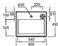
Vanity top 60 x 49 cm
