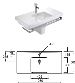
Vanity top L 105 x 50 cm E4731 - €480 incl. VAT (excluding towel rail)
