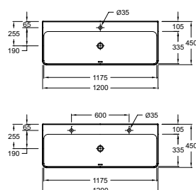
Vessel basin 120 x 45 cm Front overflow EVA112 - 1 tap hole EVA122 - 2 tap holes Starting at €918 incl. VAT
