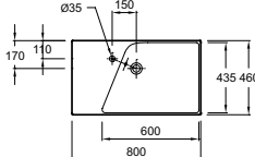
Vanity top 80 x 46 cm EXO112-Z €483 incl. VAT
