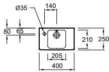
Handwash basin 40 x 25 cm E4759G - €115 incl. VAT Version with right tap hole E4799G
