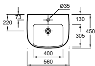
Washbasin 56 x 45 cm E4737 - €118 incl. VAT (except semi-pedestal)
