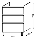
Base unit and vanity top 60 cm 3 soft-close drawers. With integrated handle. Supplied with a pair of feet (11 cm) EB847 EB2050-RA + EXAF112-Z Starting at €1.506 incl. VAT and €3.90 eco-contribution
