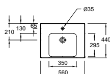
Inset vanity basin 56 x 44 cm E4756 - €217 incl. VAT
