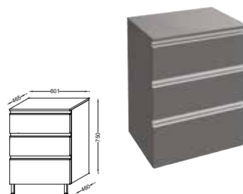
Side unit 60 cm 3 soft-close drawers. With integrated handle. Supplied with a pair of feet (11 cm) EB847 EB2065-RA Starting at €1,189 incl. VAT and €3.90 eco-contribution
