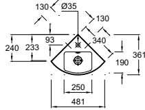
Corner handwash basin 34 x 34 cm E4733 - €102 incl. VAT
