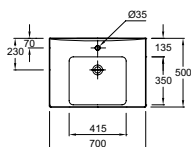
Vanity top 70 x 50 cm E4732 €360 incl. VAT
