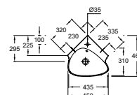
Corner handwash basin 45 x 46 cm EGL112 €325 incl. VAT
