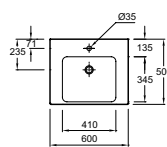
Vanity top 60 x 50 cm E4778 €327 incl. VAT
