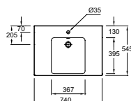
Vanity top (complies with PRM regulations) 74 x 54.5 cm E4494 - €388 incl. VAT
