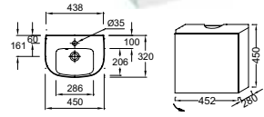
Handwash basin on cabinet L 45.2 cm EB999D + E4760 (RH hinges) EB999G + E4760 (LH hinges) €466 incl. VAT and €1.10 eco-contribution
