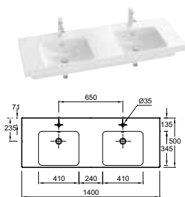
Double basin vanity top L 140 x 50 cm E4779 - €873 incl. VAT (excluding feet)
