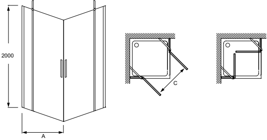
2 doors of same size 100 or 120 cm
