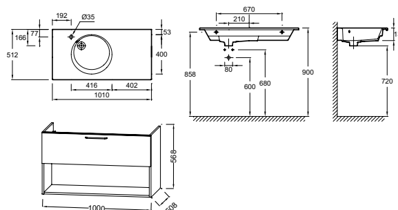
EXAU112-Z-00 Vanity top with smooth underside 101 x 51 cm
