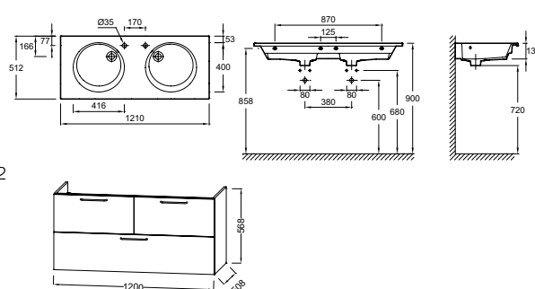
EXAT112-Z-00 Vanity top with smooth underside 121 x 51 cm
