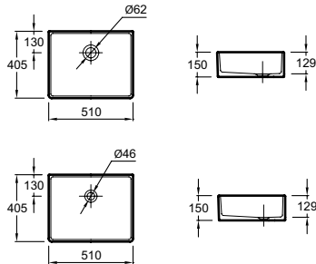
NF ESA01-00 Delta - Counter sink 50 x 40 cm no overflow, glazed on 3 sides for installation against wall. Recommended waste: Grid waste 62mm E78561. NF EVH001-00 Delta - Counter sink 50 x 40 cm without overflow, glazed on 4 sides. Recommended waste: Trap with fixed overlap cover 46mm E78293.
