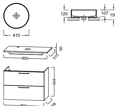
EVR002-00 Delta Pure round vessel basin in delicate ceramic Ø 41 cm, no tap hole or overflow.
