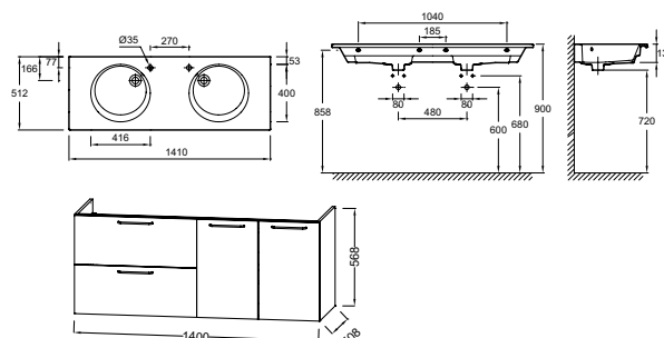
EXAS112-Z-00 Vanity top with smooth underside 141 x 51 cm
