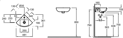
E4733-00 Odéon Up - Corner handwash basin 34 x 34 cm, 1 tap hole.
